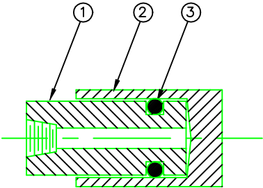
HEAD STEAM CYLINDER(No.26) (PART No.A-4240)
